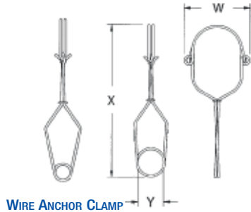
WIRE ANCHOR CLAMP
